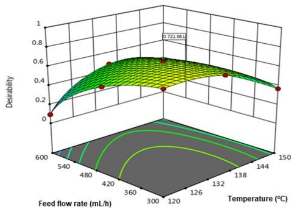
Figure 1. Process optimization response surface plot.
